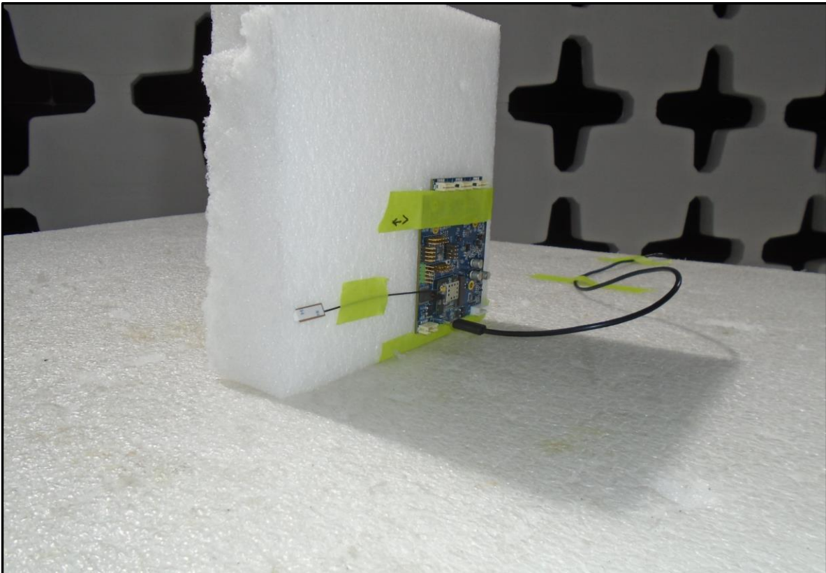
Trace ant (2)
