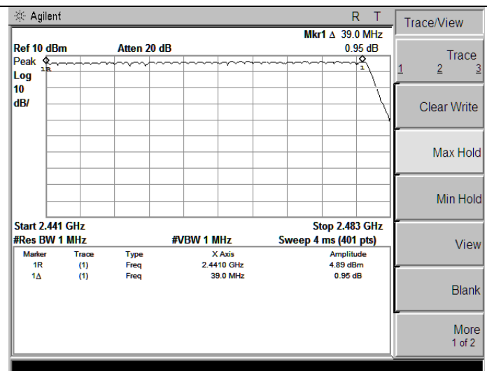
Test Plot 2 of Number of Hopping Channel(GFSK)
