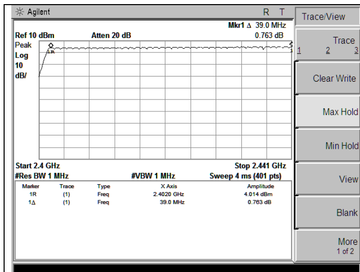
Test Plot 1 of Number of Hopping Channel(GFSK)
