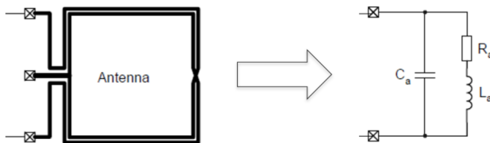
FIGURE4.2 ANTENNA EQUIVALENT CIRCUIT
