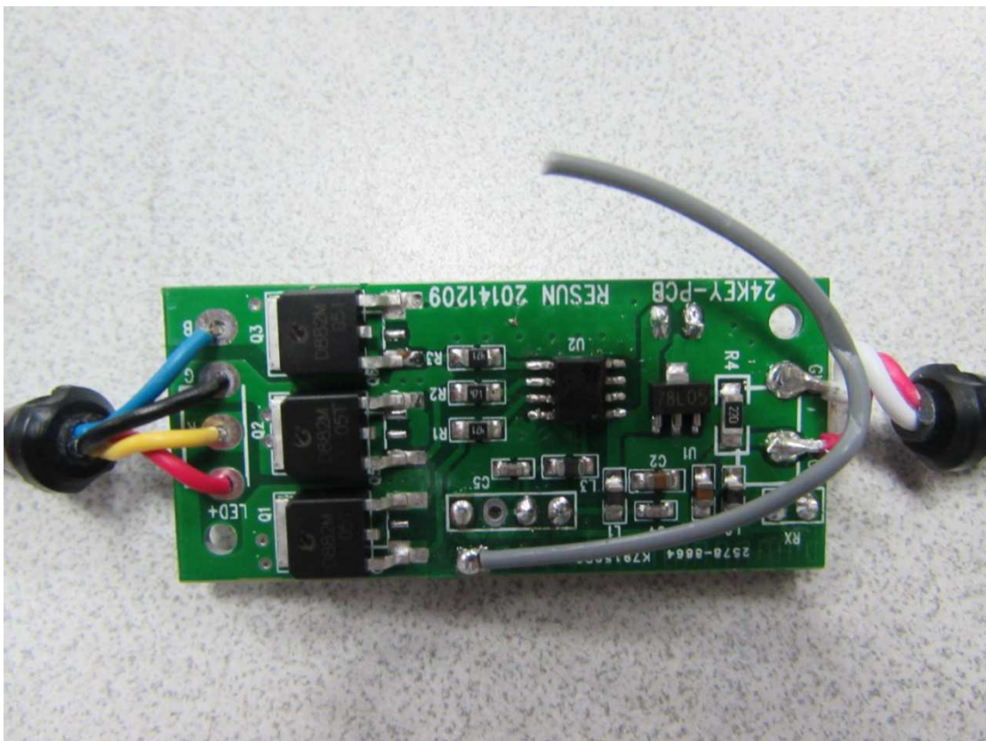
Receiver PCB view
