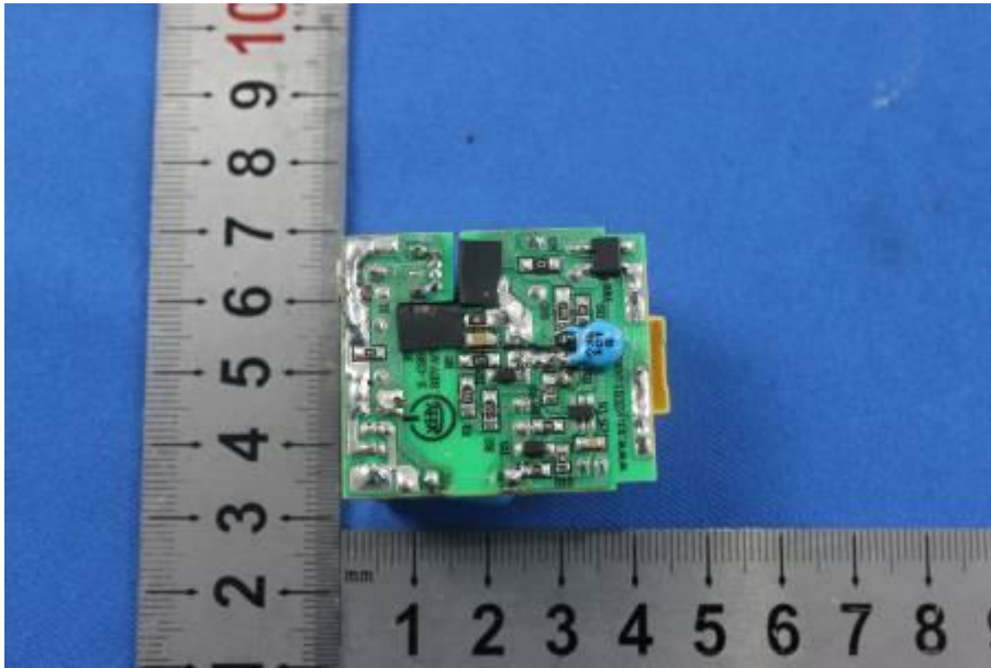
RF board and BT antenna
