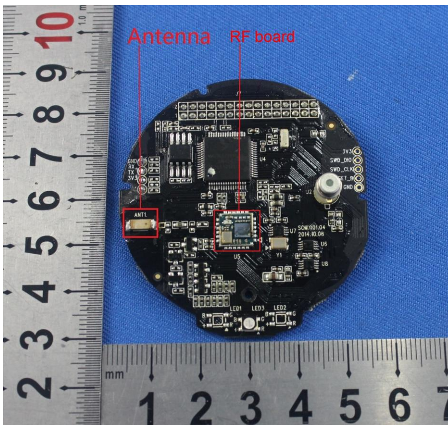
RF board and BT antenna
