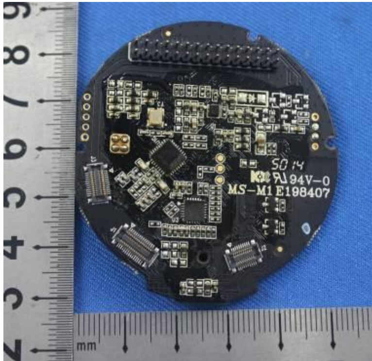
PCB in cup
