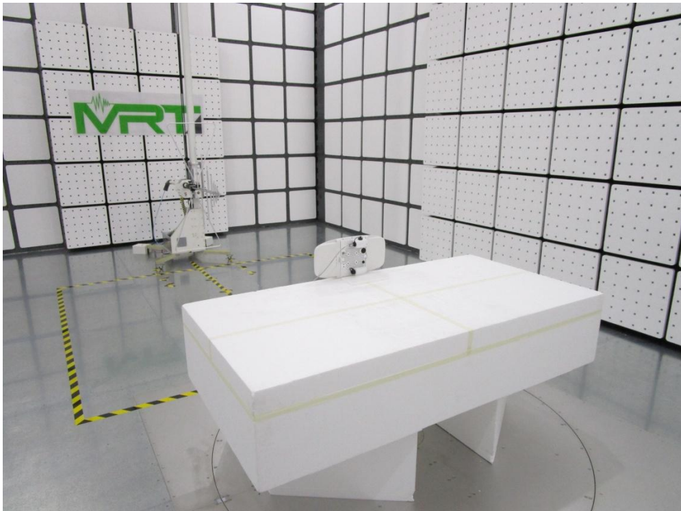
Description: Galtronics Omni Antenna Radiated Emission Test Setup for 30MHz ~ 1GHz
