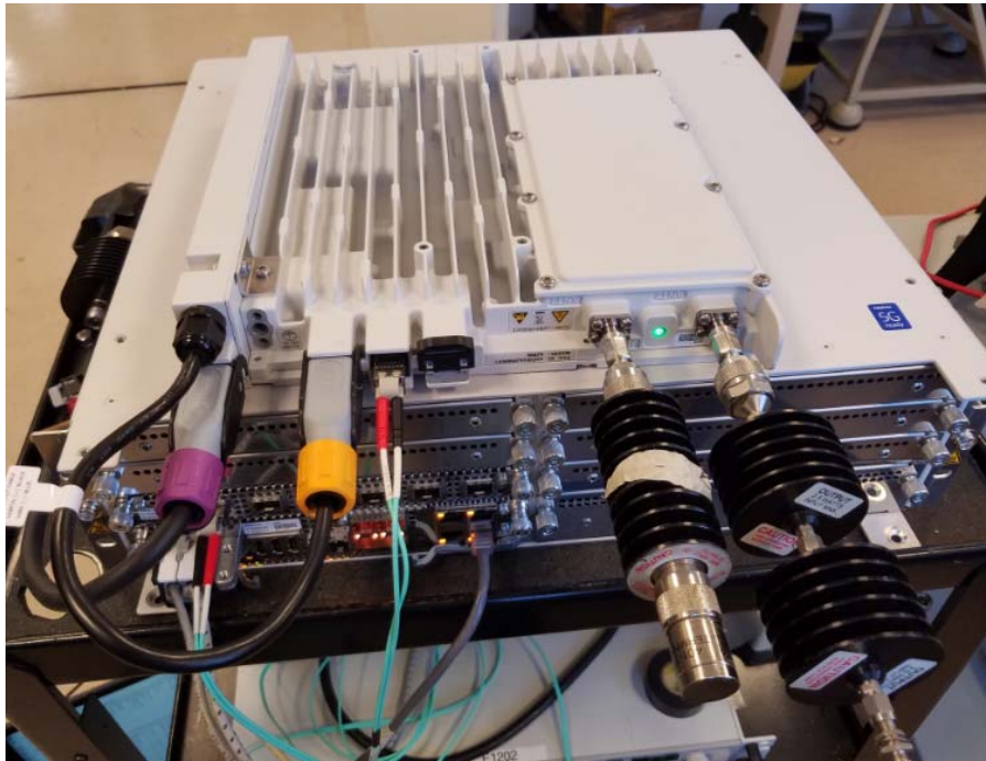
Figure 4. Setup Photo of RF Conducted Test
