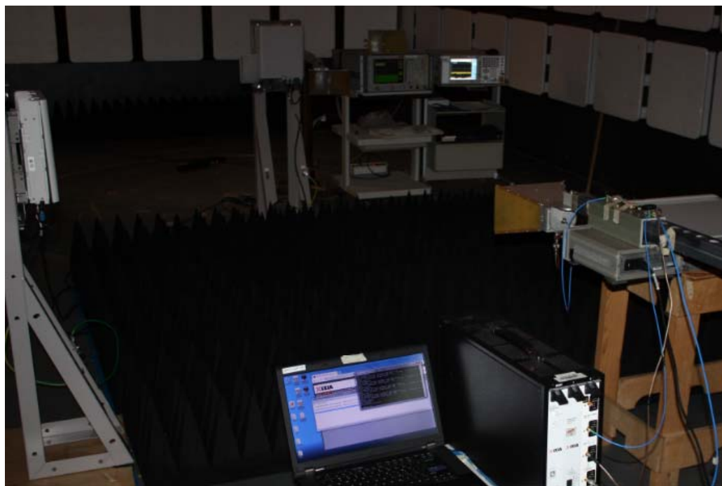
Figure 6. Setup Photos of DFS Test
