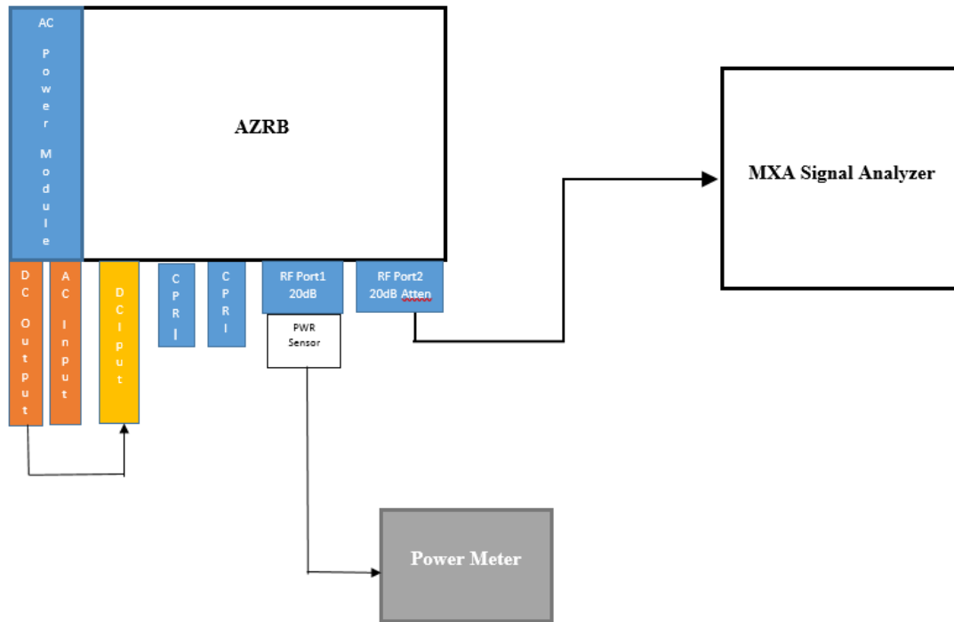
Figure 1. Setup Diagram and Photo of RF Conducted Test
