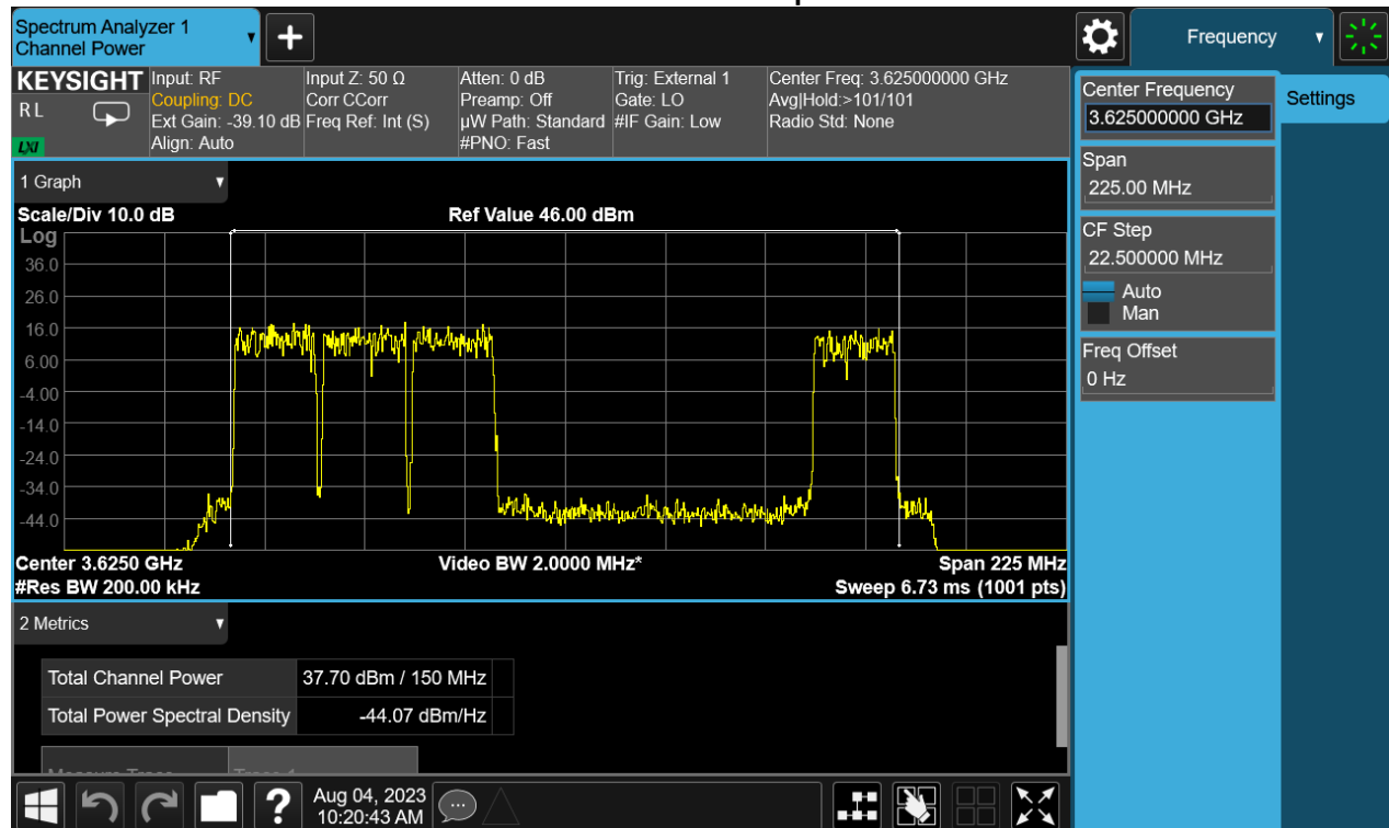
Maximum RF Conducted Output Power Plot
