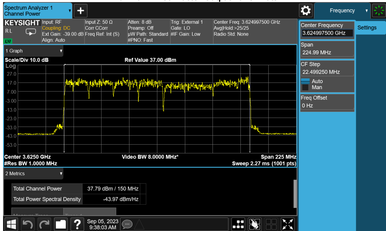
Maximum RF Conducted Output Power Plots
