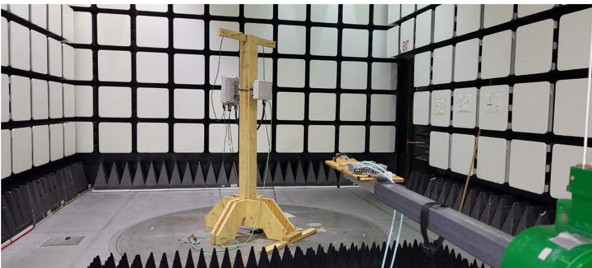
Figure 3. Photos of Radiated Tests
