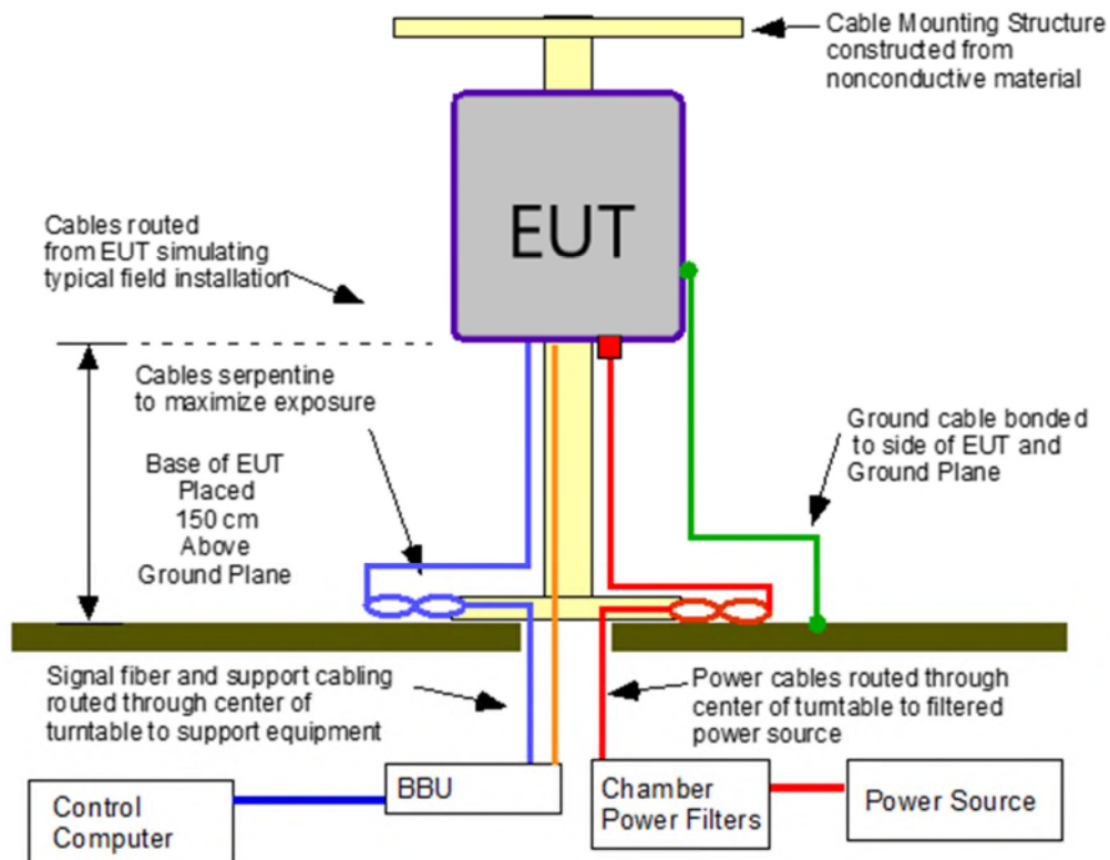
Figure 2. Test Setup for Radiated Emissions
