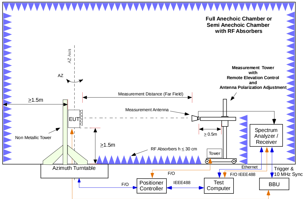
Figure 1. Test Set-Up for Measurement of Radio Transmitter Performance
