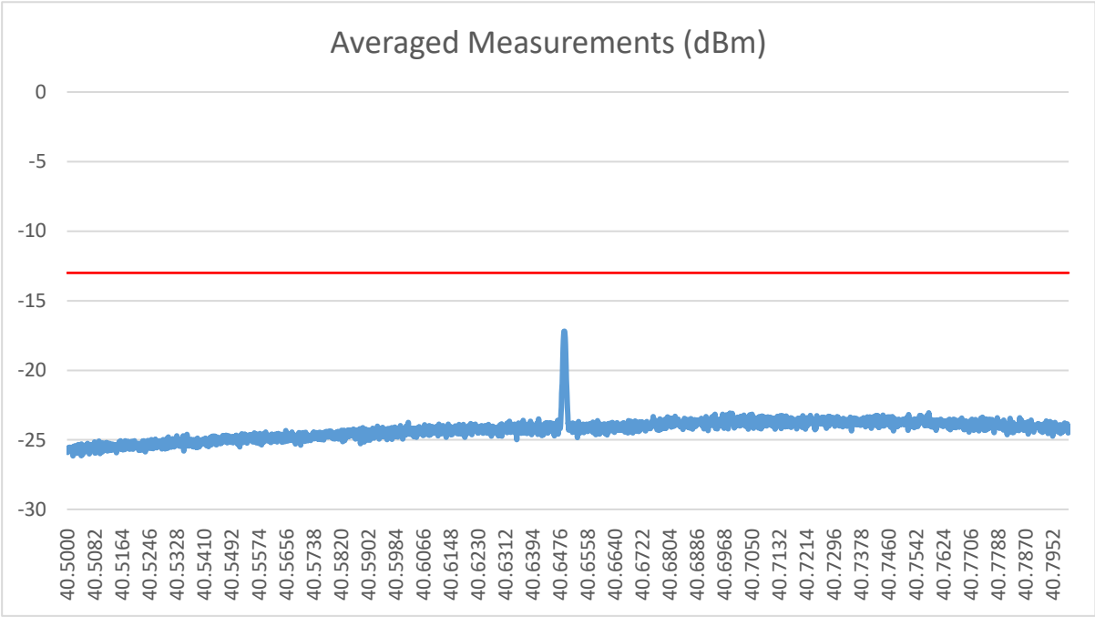
TRP Data Plot for 40.5-40.8 GHz
