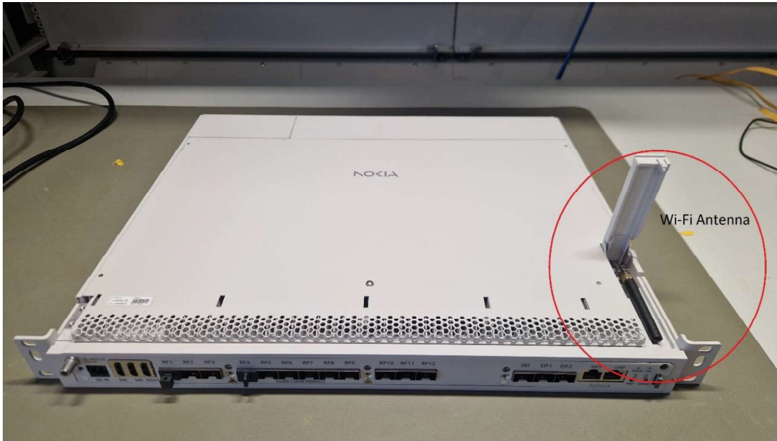
ASOH with antenna cover open
