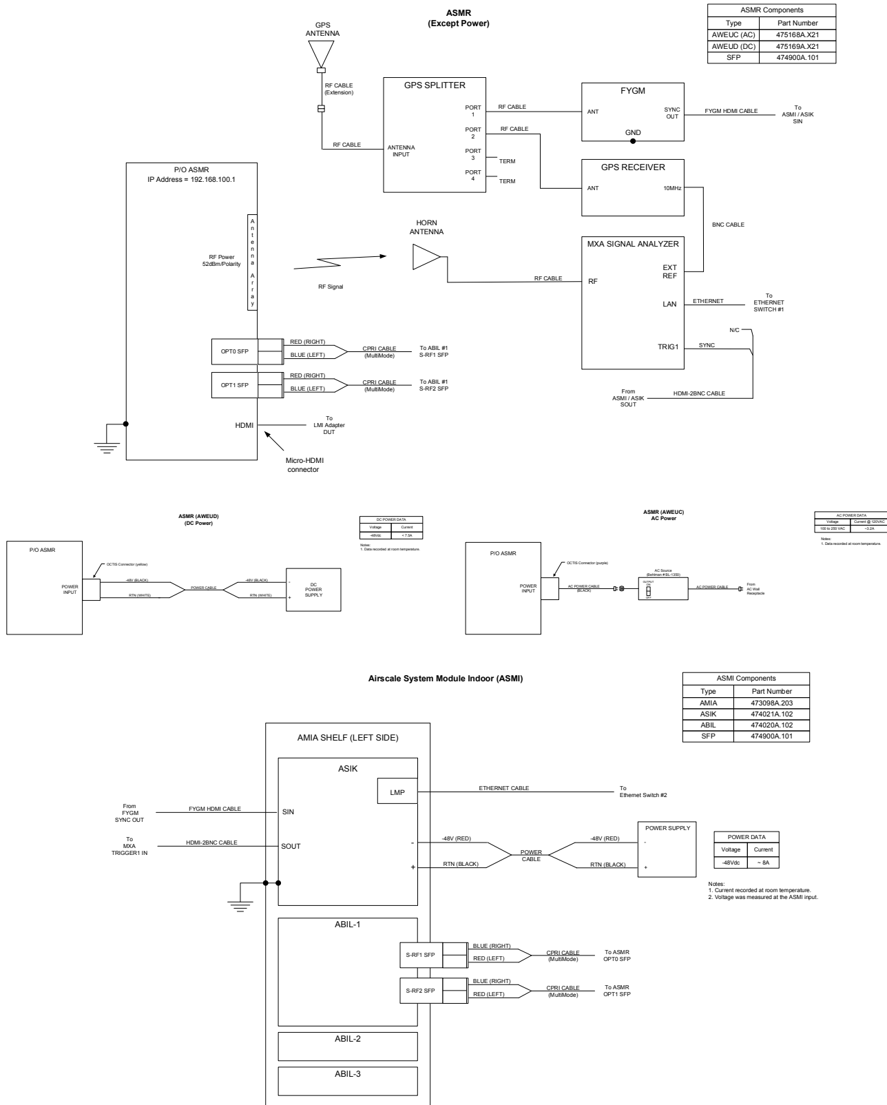
FIGURE 4.6.1: Frequency Stability Test Block Diagram
