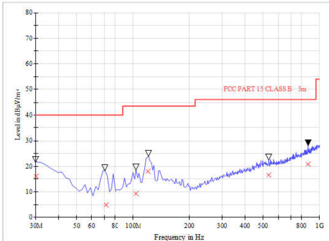
(Plot D: Test Antenna Horizontal 30M - 1G)
