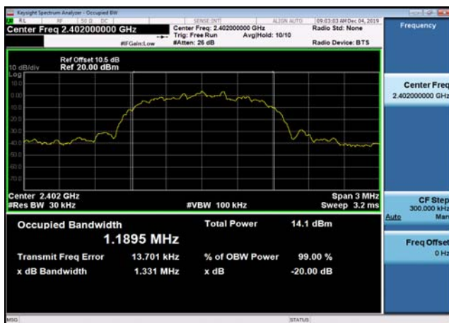
99% Bandwidth: 8DPSK,2402MHz,3DH5
