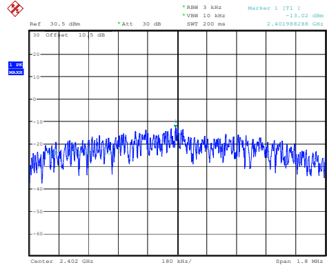
BLE_2M_Low_Channel
