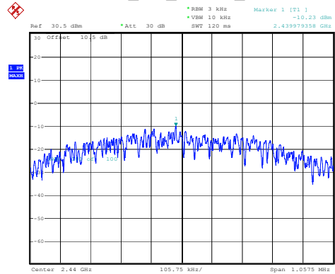
BLE_1M_Middle_Channel
