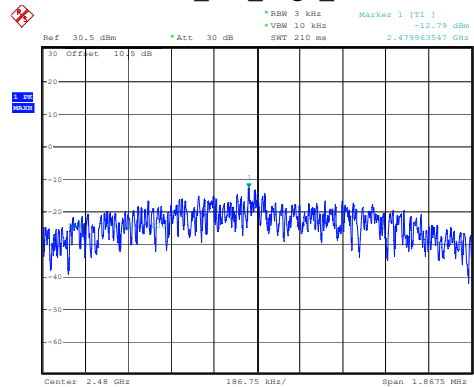
BLE_2M_High_Channel
