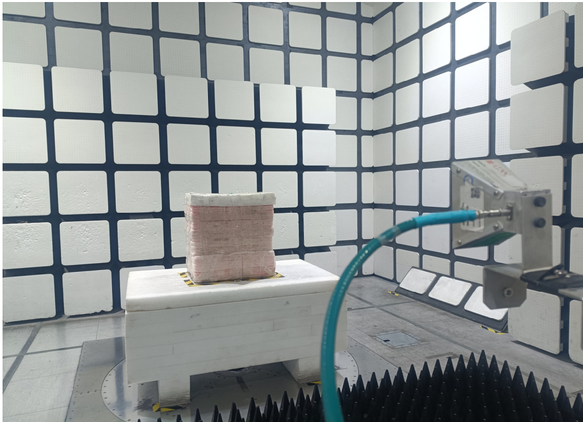
Radiated Emissions View (18-25GHz)
