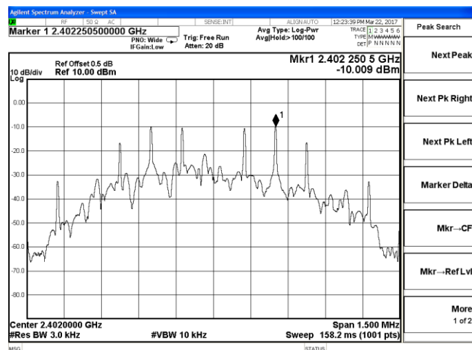
Channel 0 / 2402 MHz
