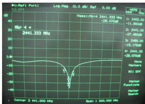
Return Loss
