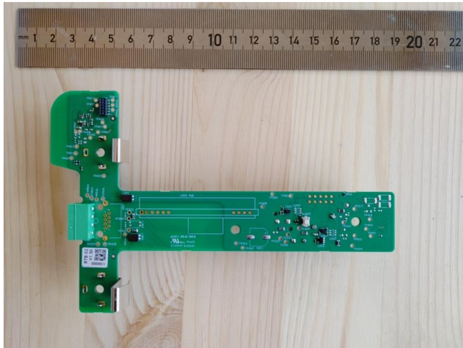
Figure 2: Photo of the PBA of INF-C361 and INF-C371, back.
