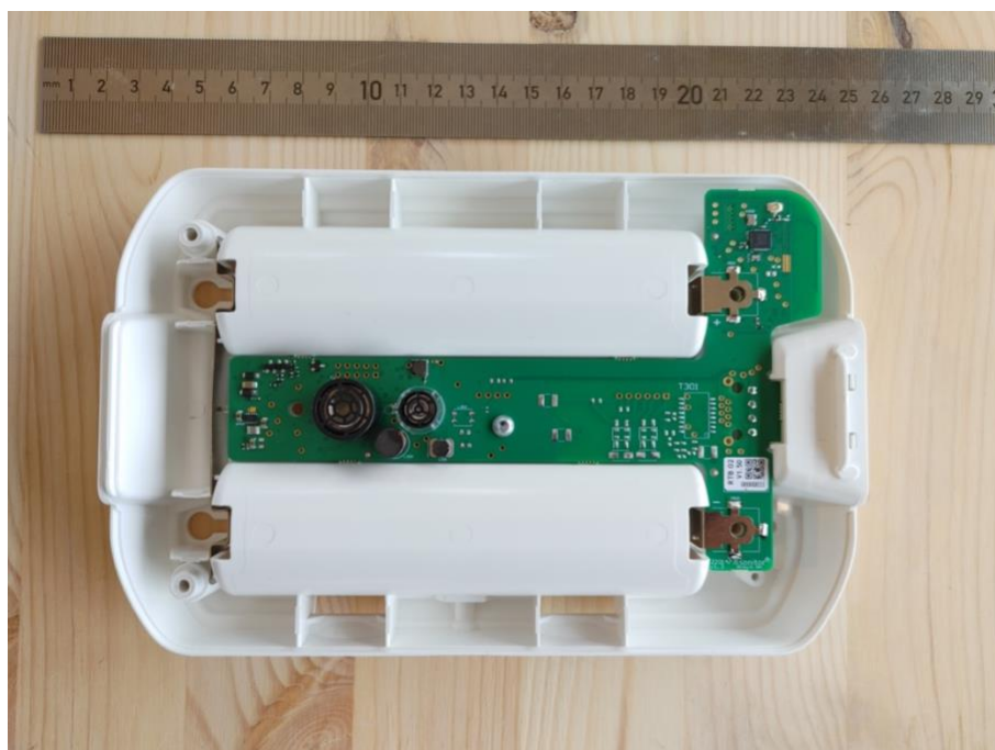
Figure 3: Photo of the PBA of INF-C361 and INF-C371, mounted inside the housing.
