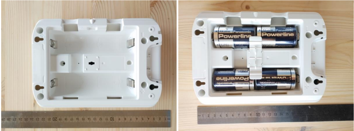
Figure 4: Photo of the battery compartment empty (left) and with batteries (right).
