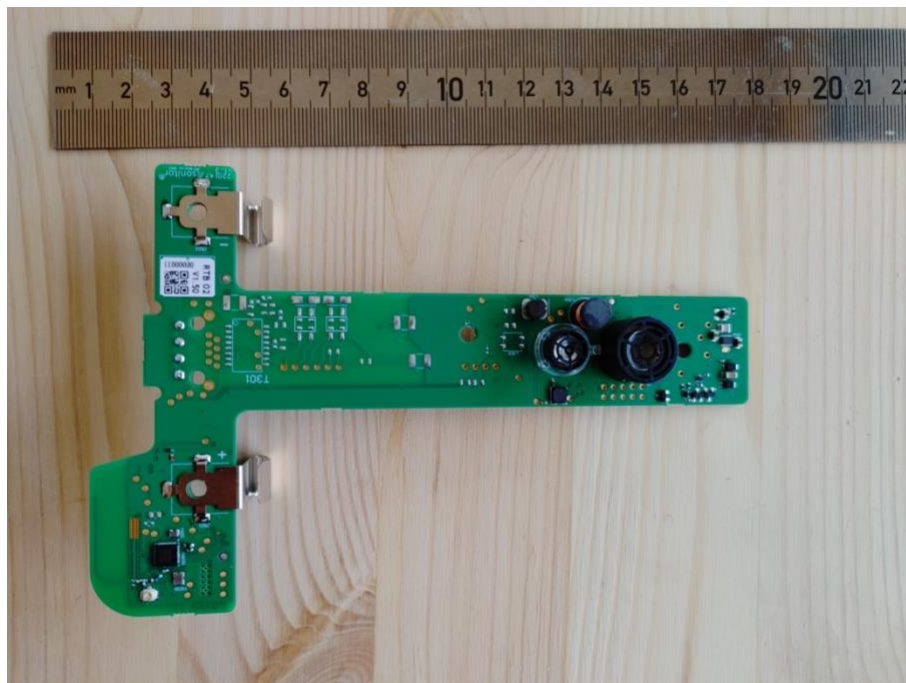
Figure 1: Photo of the PBA of INF-C361 and INF-C371, front.
