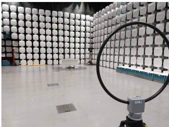
Radiated Emissions < 30MHz
