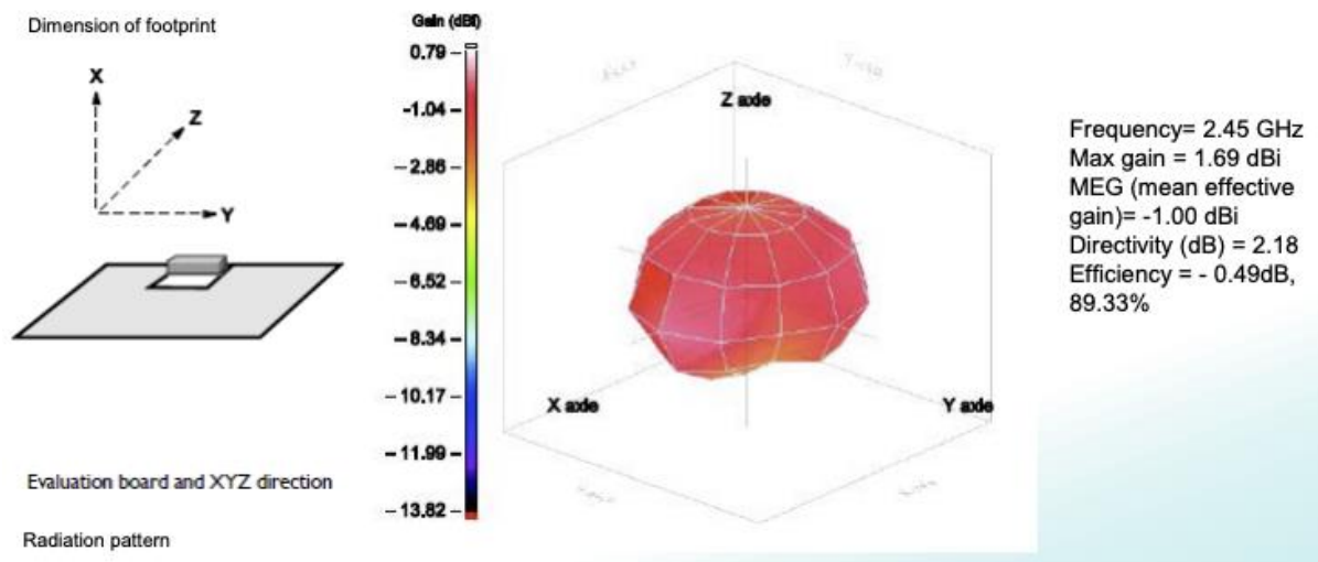
Figure 1: Extractions from the datasheet of ANT3216A063R2400A.
