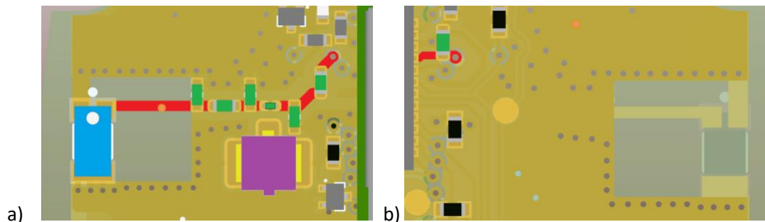
Figure 2: Details from the PBA where a) the chip antenna is colored blue and tuning components green. In b) the opposite side of the board is shown where also one tuning component is present.
