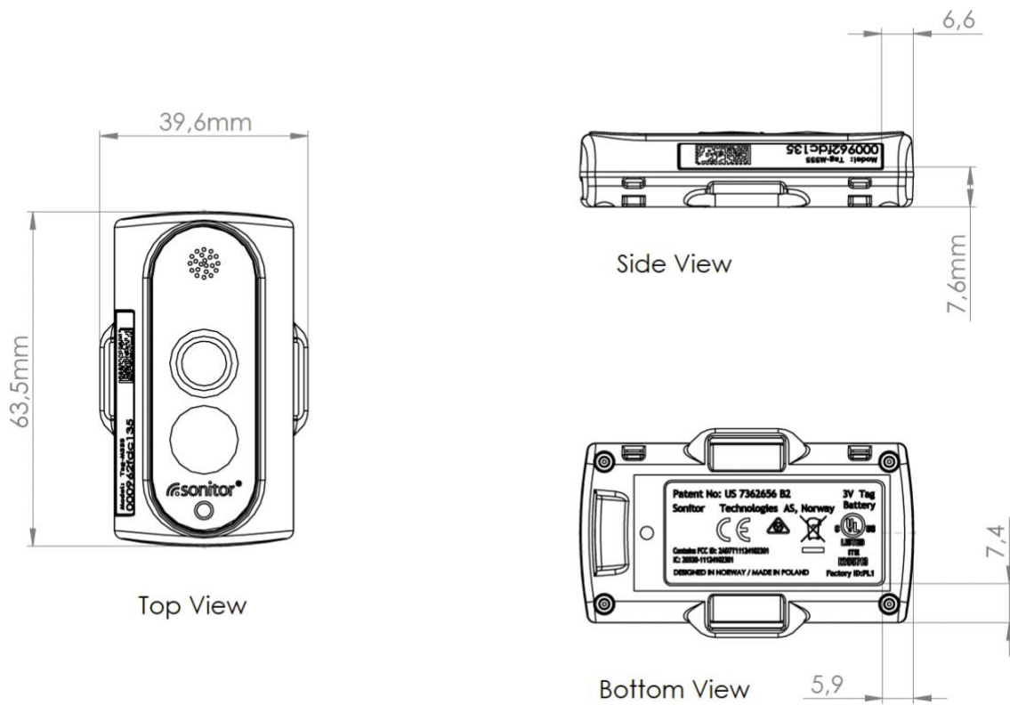
Figure 22: Placement of labels on the side and bottom of the tag.
