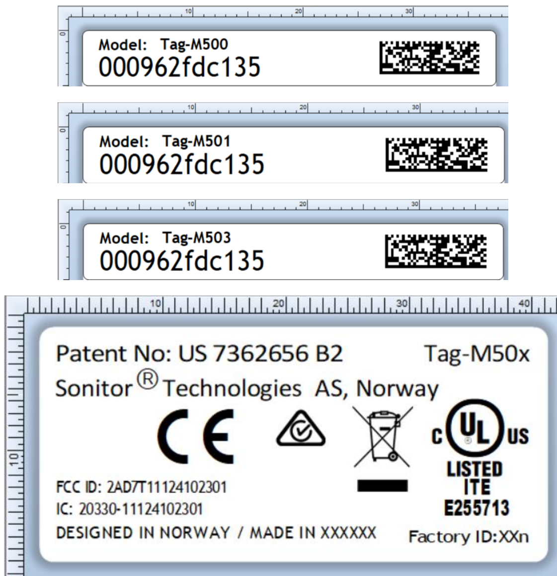
Figure 1: The smaller label (upper image) and the larger label (lower image) for Tag-M50X.
