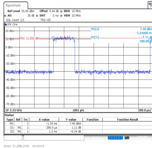
NTNV-11AX40SISO-Ant1-5230
