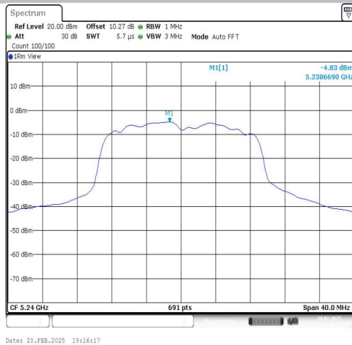
11AX20SISO-Ant1-5240-PASS
