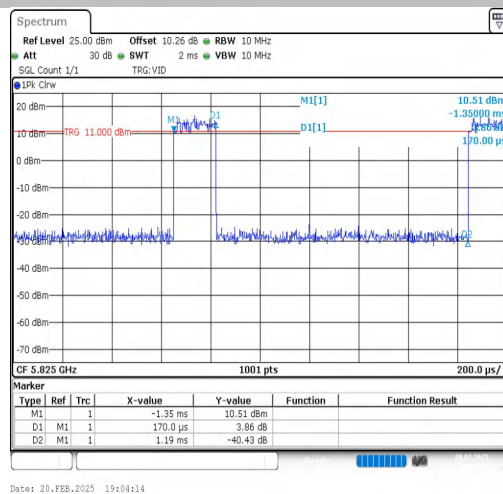
NTNV-11AC20SISO-Ant1-5825
