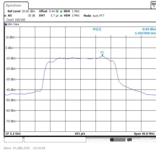
11AX20SISO-Ant1-5200-PASS
