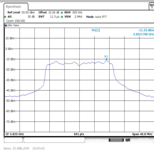
11AX20SISO-Ant1-5825-PASS
