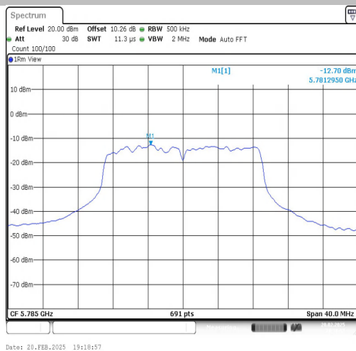
11AX20SISO-Ant1-5785-PASS
