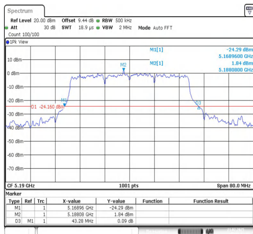
11AX40SISO-Ant1-5190
