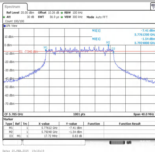
11AX20SISO-Ant1-5785-PASS
