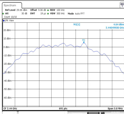
BLE_2M-Ant1-2440-0~Reference-PASS
