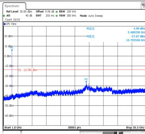
BLE_2M-Ant1-2480-0~Reference-PASS
