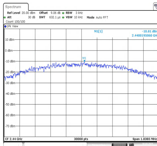
BLE_1M-Ant1-2440-PASS
