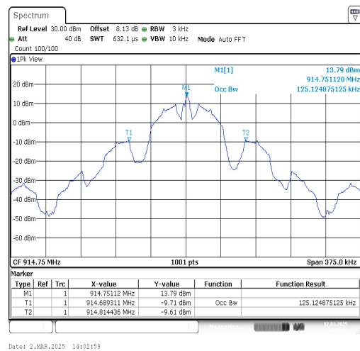
RFID-Ant1-914.75
