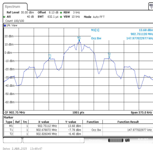
RFID-Ant1-902.75
