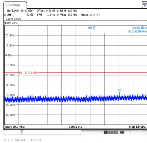
3DH5-Ant1-2402-30~1000-PASS
