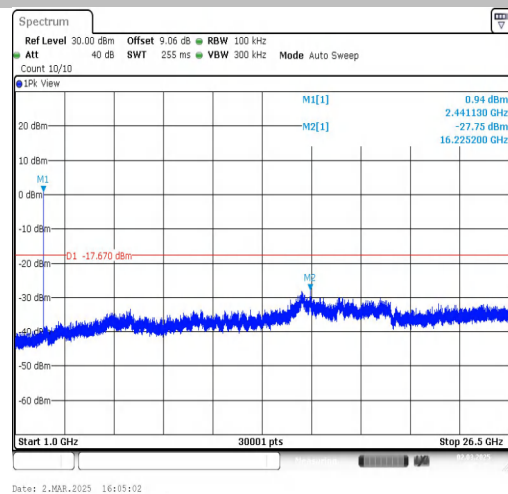
3DH5-Ant1-2441-1000~26500-PASS
