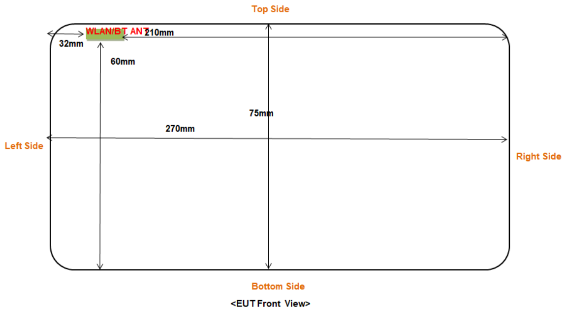
Fig 7.2 Block Diagram for EUT Antenna Position EUT Size: Long*Width*Height=270mm*75mm *40mm
