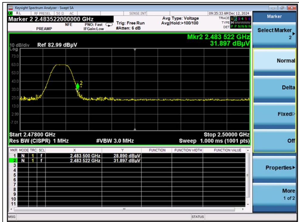
(PEAK, Channel 3)
