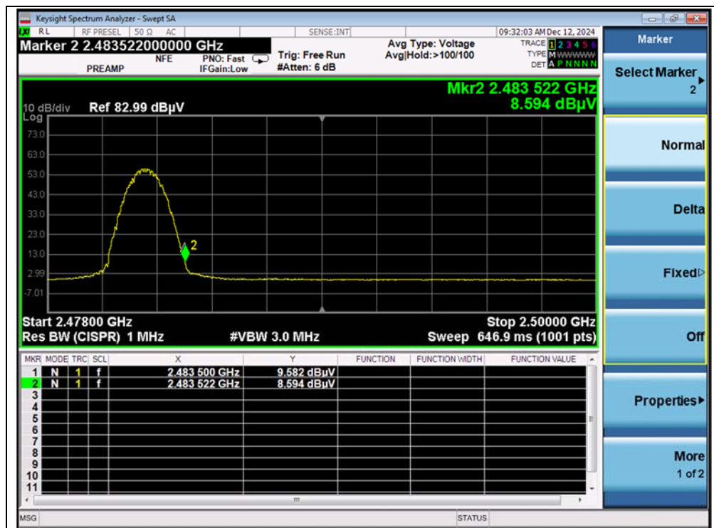
(AVERAGE, Channel 3)
