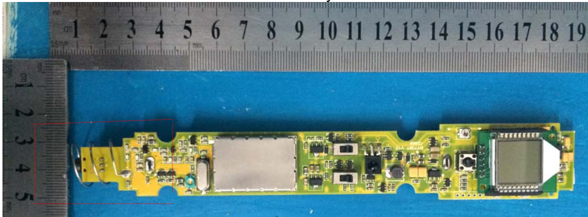
U-2100BT with PCB Layout's Antenna
