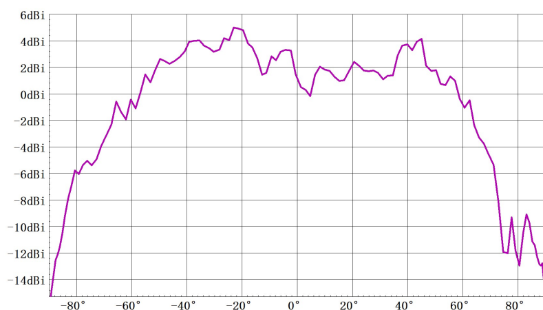
俯仰面方向图 (TX0) Freq:57.0GHz
