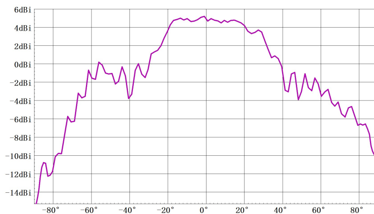
方位面方向图 (TX1) Freq:62.0GHz
