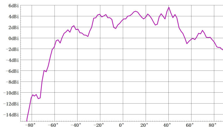
俯仰面方向图 (TX1) Freq:60.0GHz
