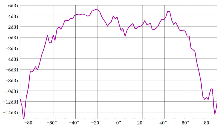
俯仰面方向图 (TX0) Freq:62.0GHz
