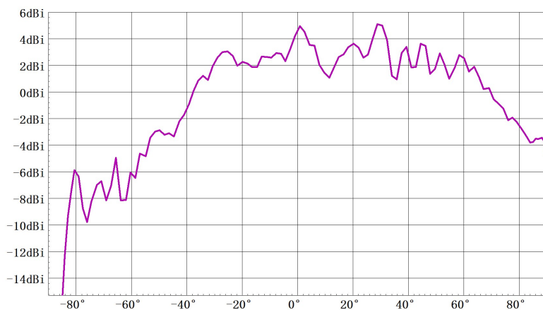
俯仰面方向图 (TX1) Freq:58.0GHz
