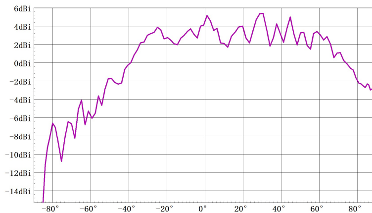
俯仰面方向图 (TX1) Freq:61.0GHz
