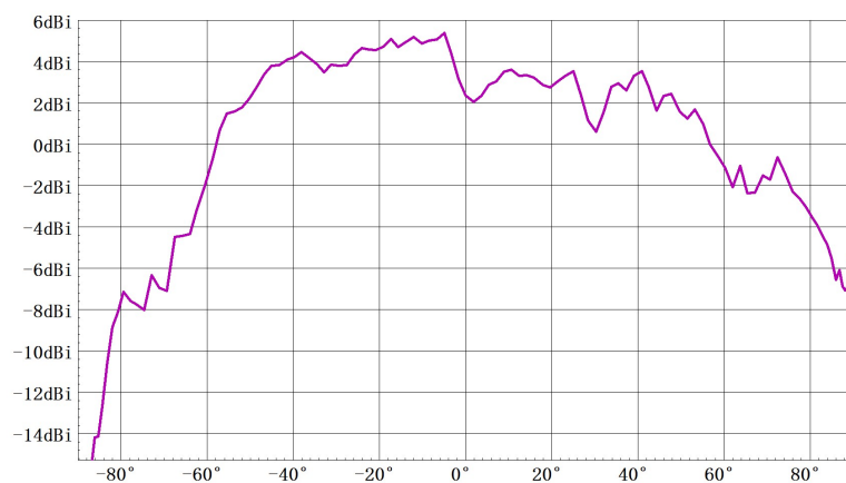
俯仰面方向图 (TX0) Freq:59.0GHz
