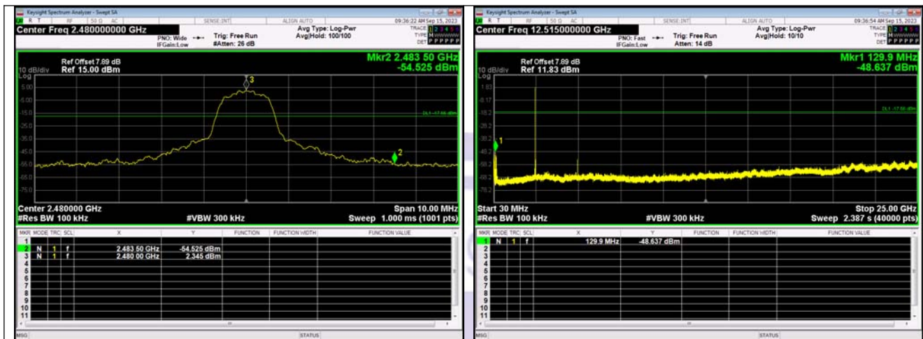
Out Of Band Emission 8DPSK_3-DH1_Channel 78
