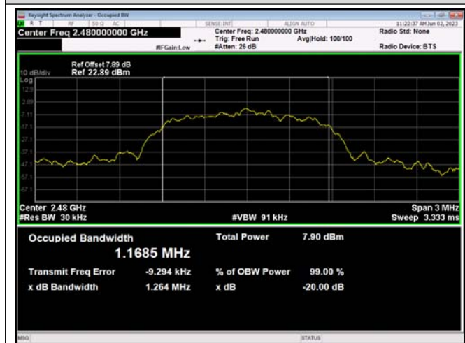
8DPSK_3-DH1_Channel 78
