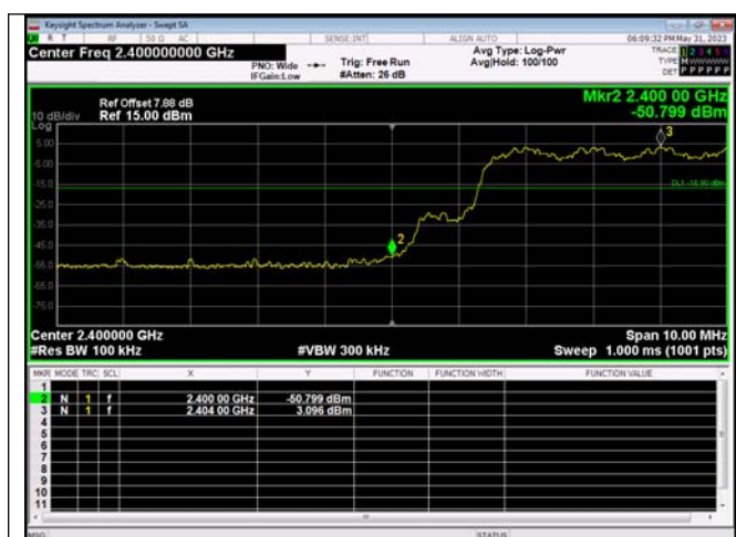
Out Of Band Emission(Left) 8DPSK_3-DH1_Channel Hopping
