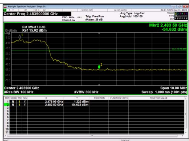
Out Of Band Emission(Right) 8DPSK_3-DH1_Channel Hopping
