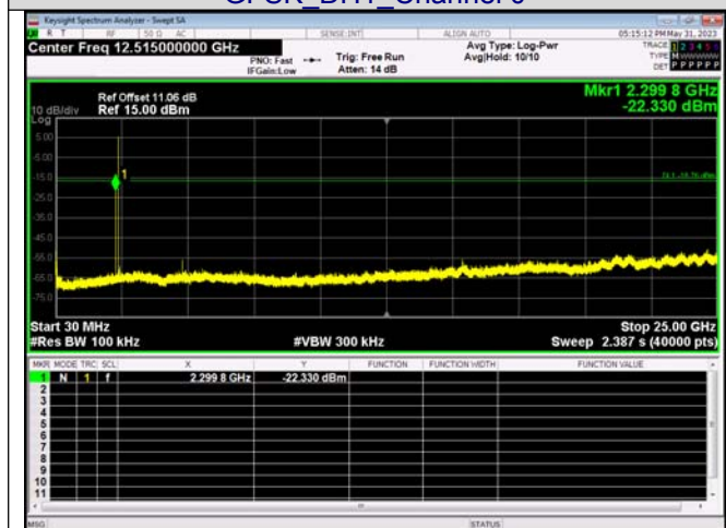
Spurious Emission GFSK_DH1_Channel 0
