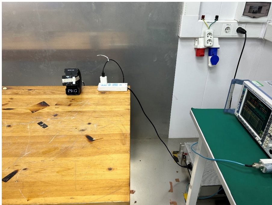
Conducted emissions(For BT)
