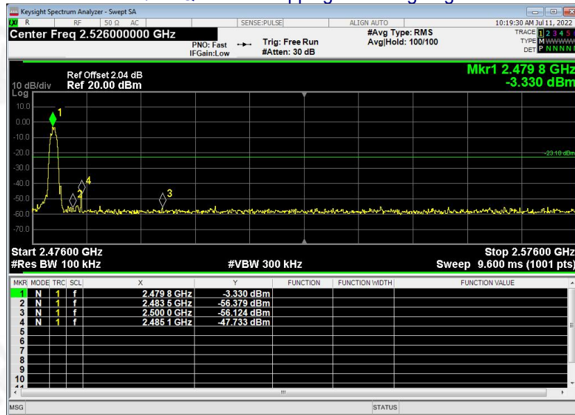
\pi/4 -DQPSK No-hopping Band edge-right side
