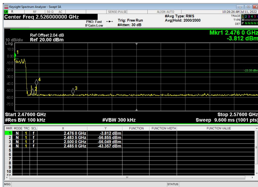
\pi/4 -DQPSK Hopping Band edge-right side
