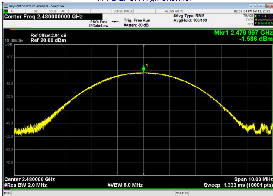
\pi/4 -DQPSK High Channel
