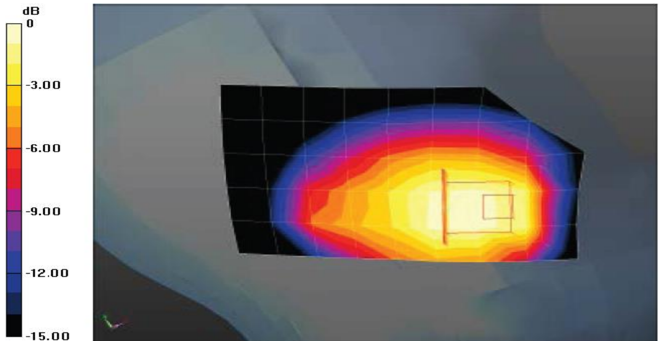
Plot 2: Body Wrist Worn (GSM850 GPRS 4TS Middle Channel)
