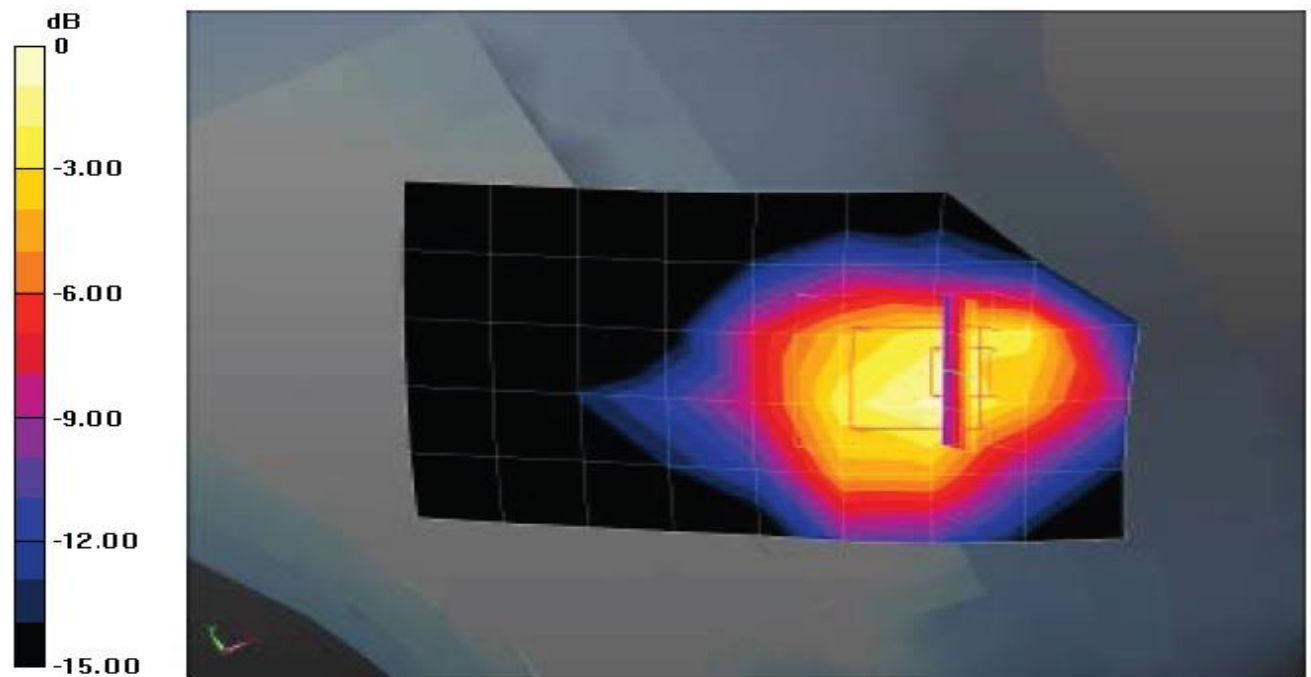
Plot 4: Body Wrist Worn (GSM1900 GPRS 4TS Middle Channel)
