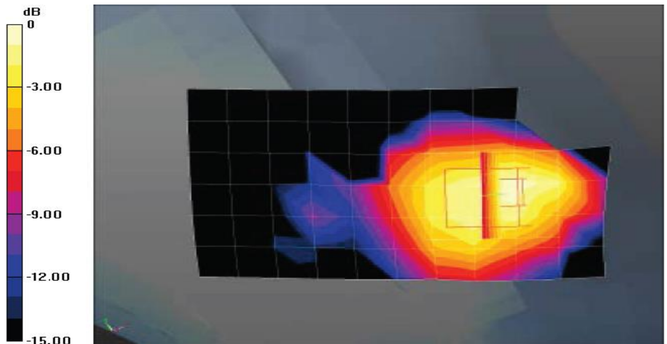
Plot 6: Body Wrist Worn (WiFi2450 Middle Channel-Channel 6-2437MHz (1Mbps))
