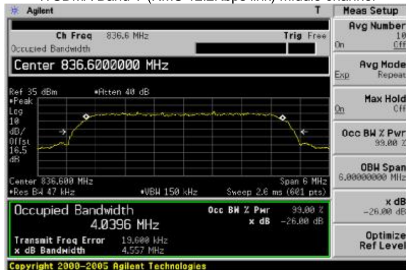
WCDMA Band V (RMC 12.2Kbps link) Middle channel
