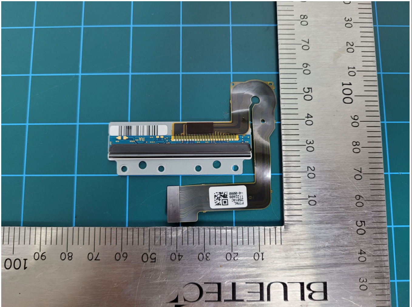
Sub board_Front
