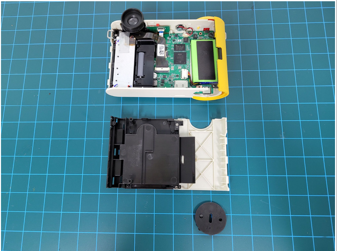
Internal Photo
