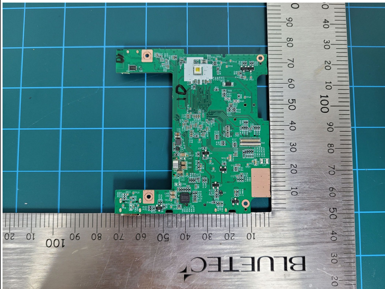
Main PCB_Rear
