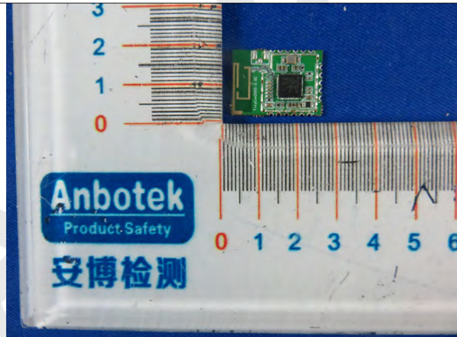
6. Figure PCB of the EUT-Front View
