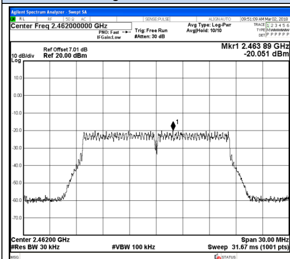
802.11g Chain 0-High channel
