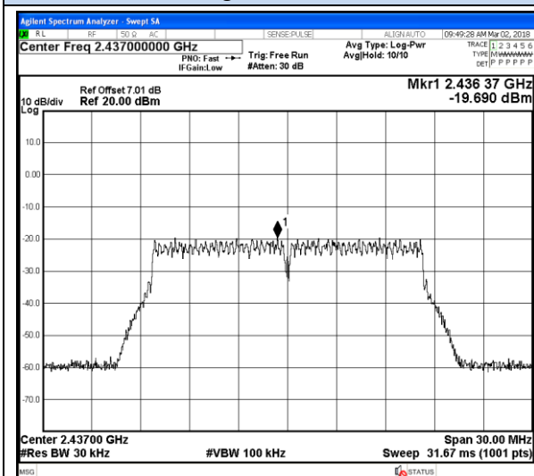
802.11g Chain 0-Middle channel
