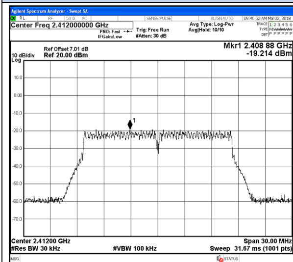
802.11g Chain 0-Low channel
