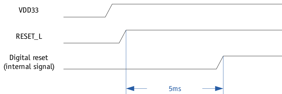
Figure 7-1. Power on sequencing for the AR9331
