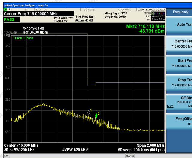
Band12-10MHz-16QAM-23130-1RB#49
