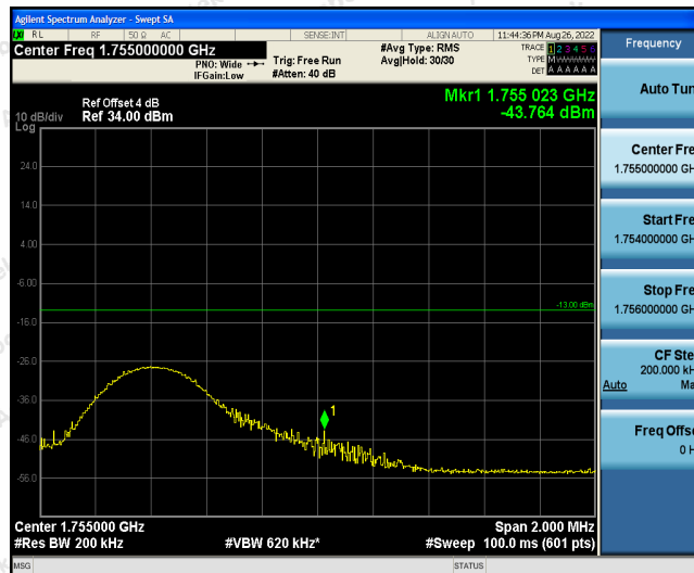
Band4-10MHz-QPSK-20350-1RB#49
