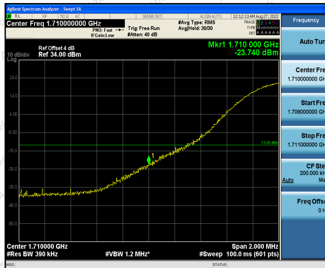
Band4-20MHz-16QAM-20050-1RB#99
