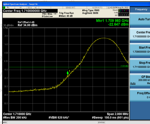
Band4-10MHz-QPSK-20000-1RB#49
