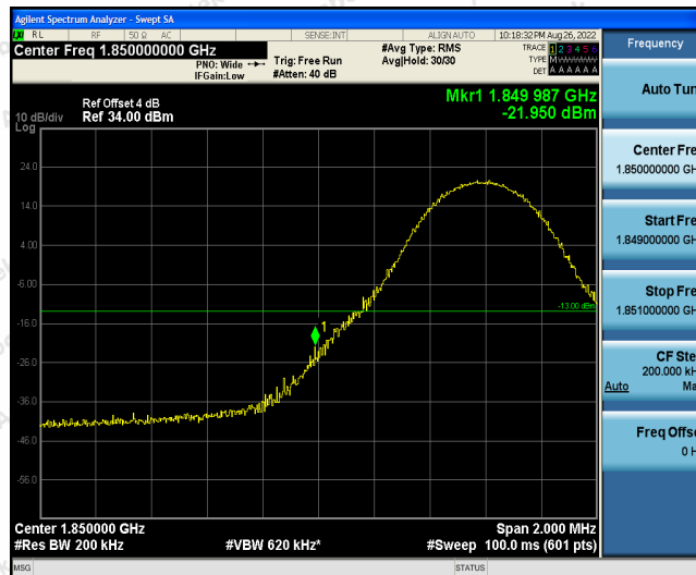
Band2-10MHz-16QAM-18650-1RB#49
