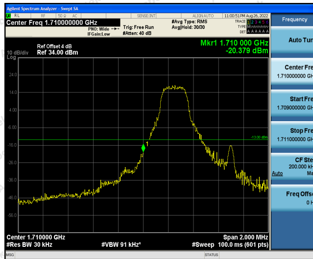
Band4-1.4MHz-QPSK-19957-1RB#5
