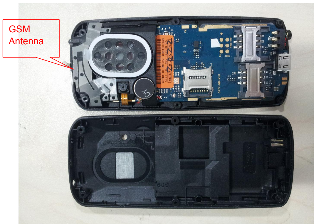
Antenna Location
