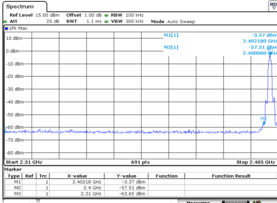
CH00 Bandedge (no hopping mode)
