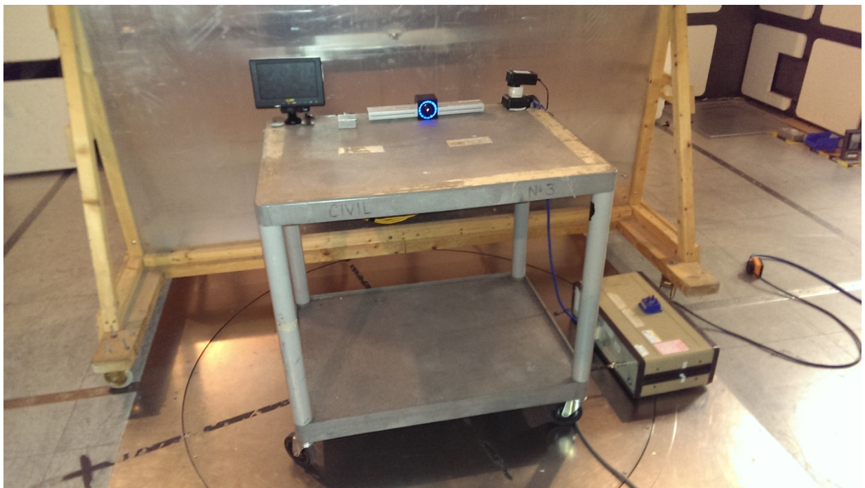
Conducted Emissions
