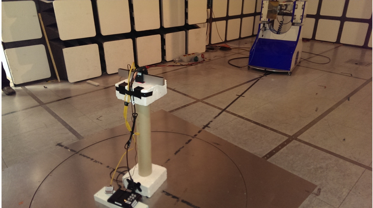
Radiated Emissions 30MHz-1GHz
