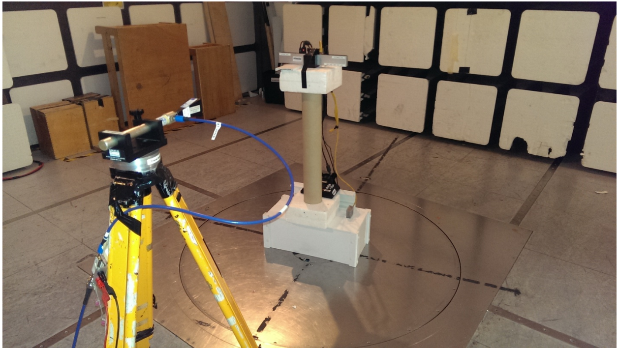
Radiated Emissions above 18GHz
