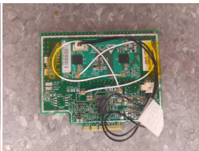
Photograph 7.7.1 Antenna assembly
