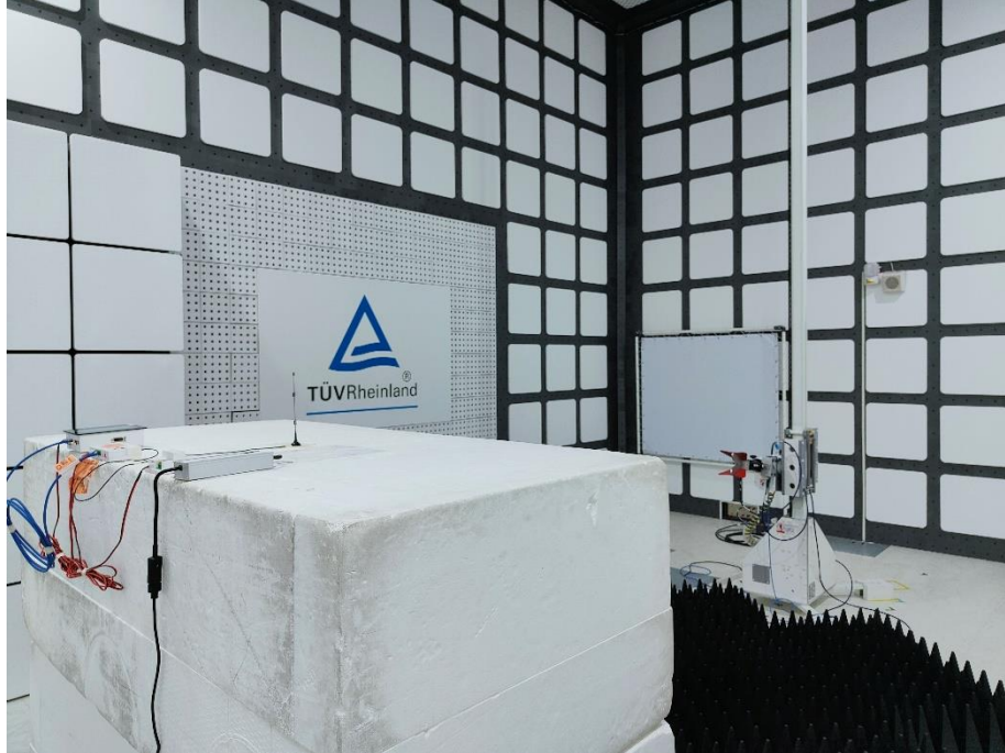
Photograph 11: Test Setup for Spurious Emissions (Back View 3)
